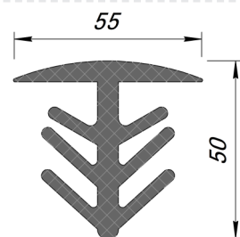
SD108-102
