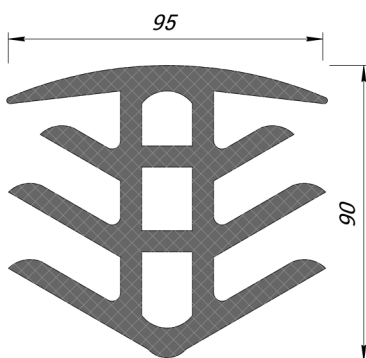
SD102-102
