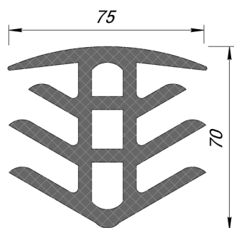
SD108-103
