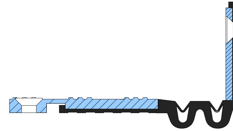
Acara Hydro HD121-100-E
